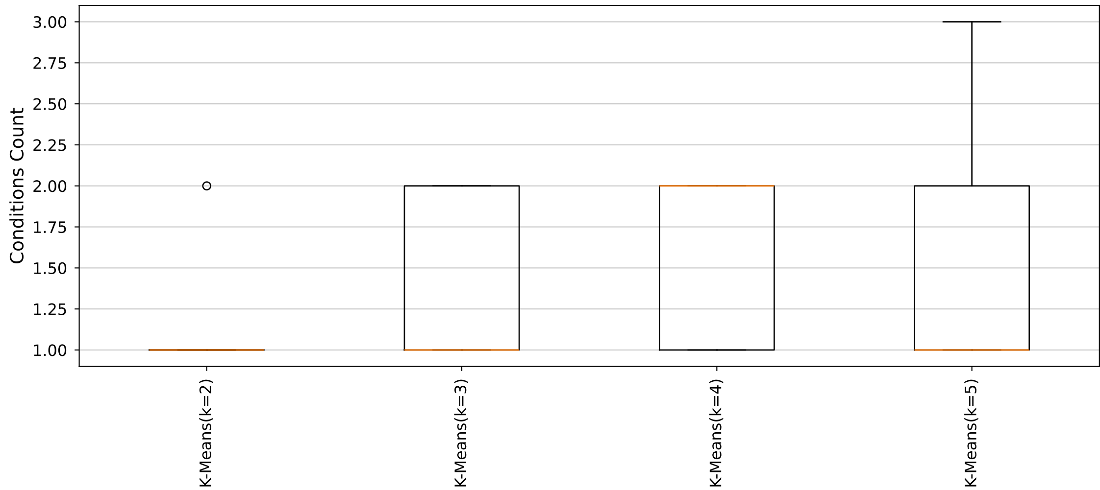
YARA Rules Conditions Count Distribution (Cluster44_Size5 dataset)
